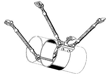
Fixed Point (trestle arrangement)
